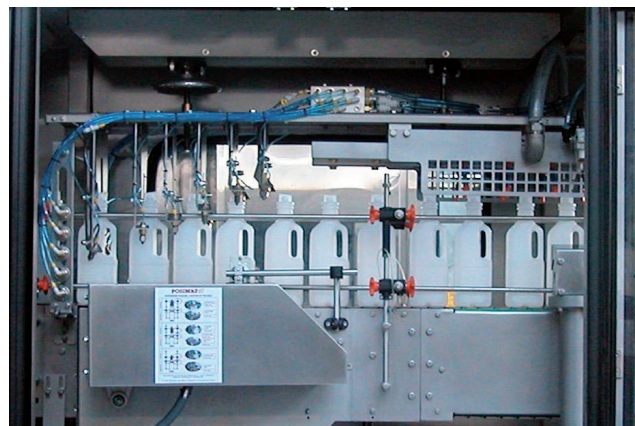
Inside of high-speed water RINSER Cleaning the outside of the bottle or jar
