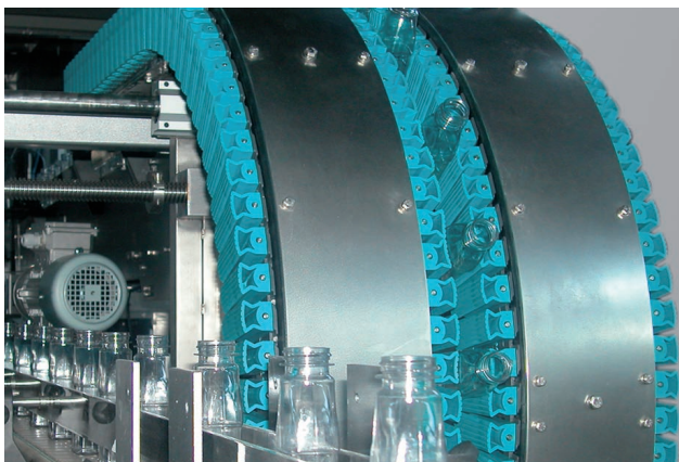
Inside of high-speed air RINSER Cleaning the inside of the bottle or jar
